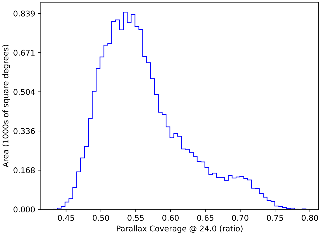
too_elab_r8_d2_gz_v3.4_10yrs WFD: Parallax Coverage @ 24.0
