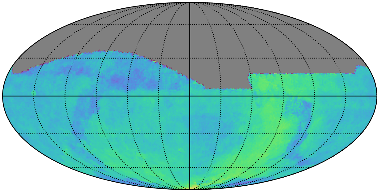
too_elab_r8_d2_gz_v3.4_10yrs All sky: Parallax Coverage @ 24.0
