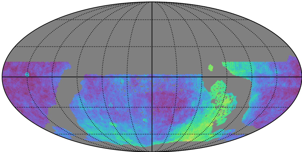
too_elab_r8_d2_gz_v3.4_10yrs WFD: Parallax Coverage @ 22.4
