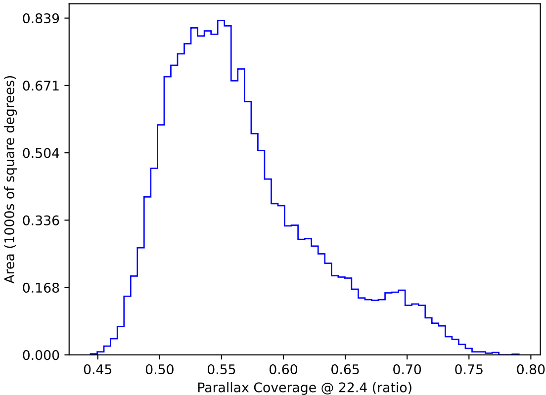
too_elab_r8_d2_gz_v3.4_10yrs WFD: Parallax Coverage @ 22.4
