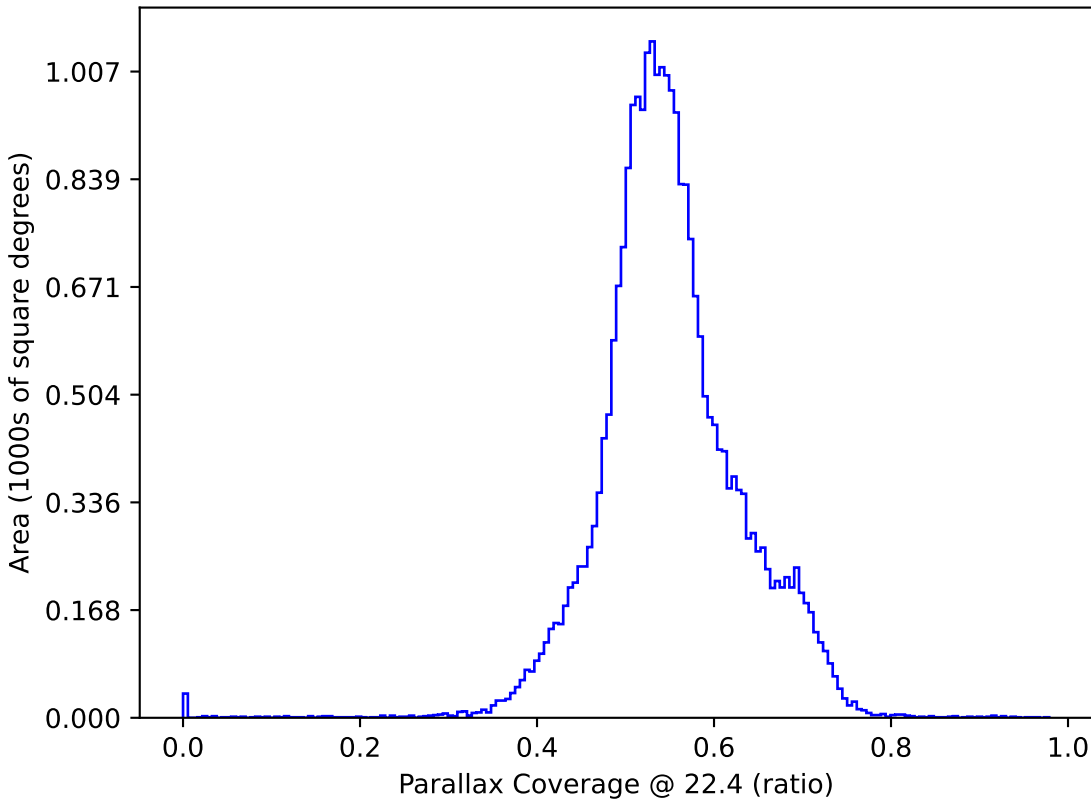
too_elab_r8_d2_gz_v3.4_10yrs All sky: Parallax Coverage @ 22.4
