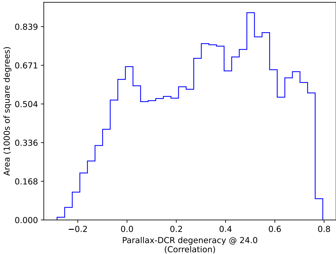
too_elab_r8_d2_gz_v3.4_10yrs WFD: Parallax-DCR degeneracy @ 24.0
