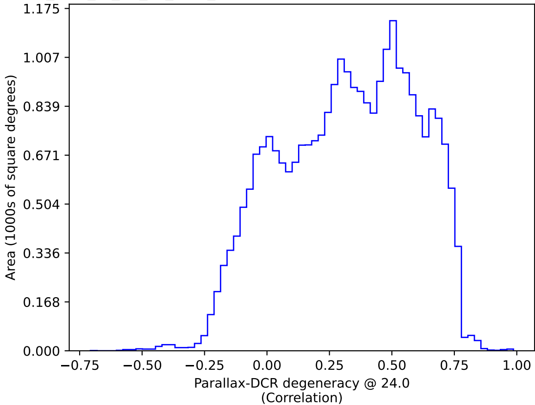
too_elab_r8_d2_gz_v3.4_10yrs All sky: Parallax-DCR degeneracy @ 24.0
