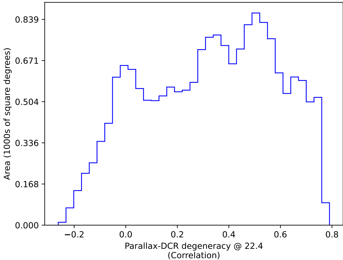
too_elab_r8_d2_gz_v3.4_10yrs WFD: Parallax-DCR degeneracy @ 22.4
