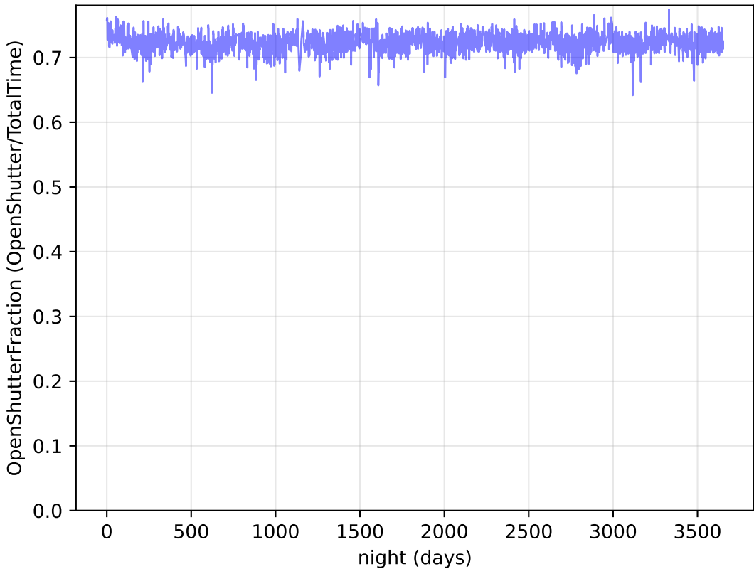
too_elab_r8_d2_gz_v3.4_10yrs Per night: OpenShutterFraction
