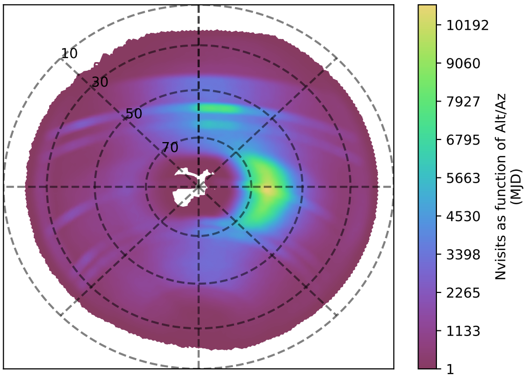
too_elab_r8_d2_gz_v3.4_10yrs all bands: Nvisits as function of Alt/Az
