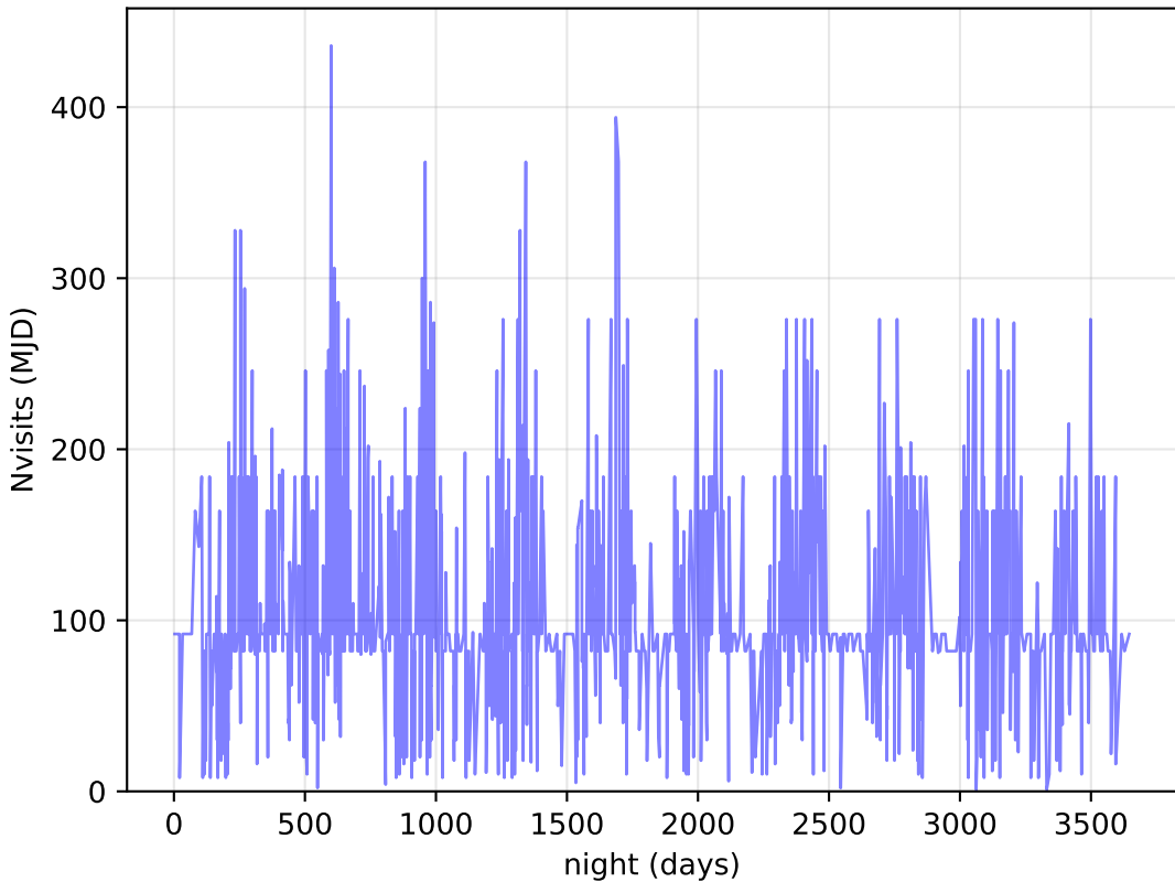
too_elab_r8_d2_gz_v3.4_10yrs DDF: Nvisits
