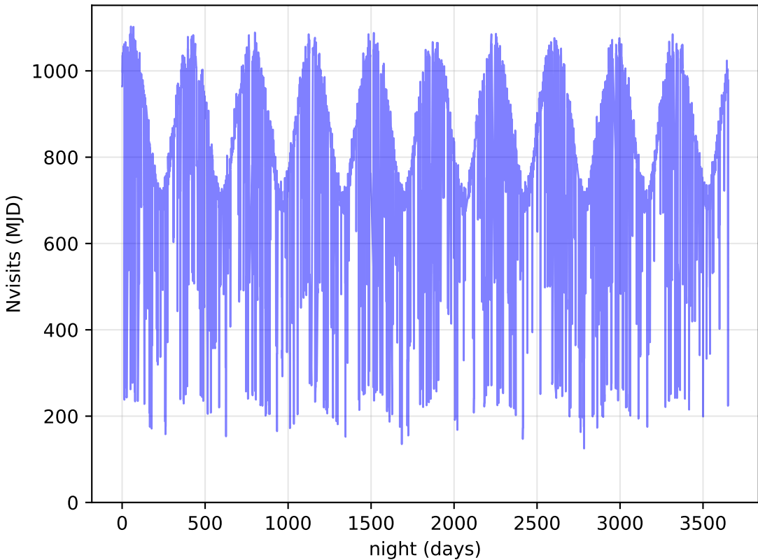
too_elab_r8_d2_gz_v3.4_10yrs All visits: Nvisits
