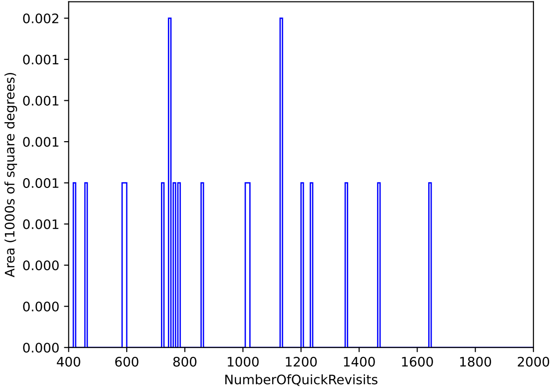
too_elab_r8_d2_gz_v3.4_10yrs WFD: NumberOfQuickRevisits
