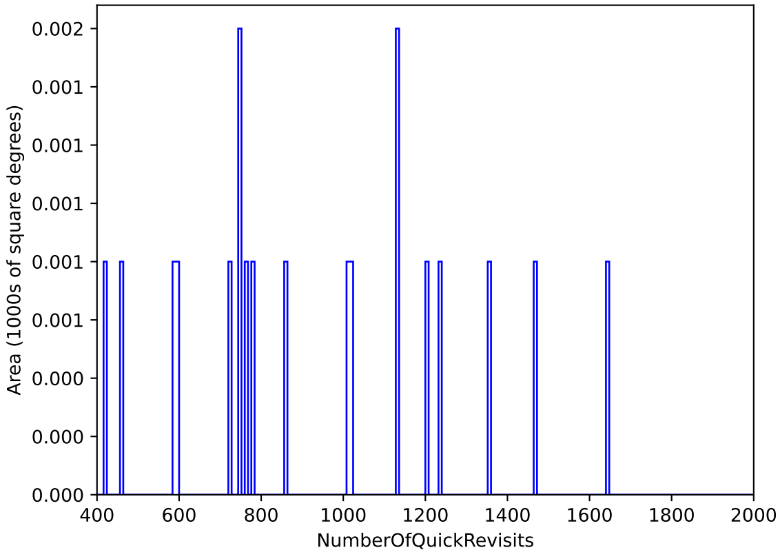
too_elab_r8_d2_gz_v3.4_10yrs All sky: NumberOfQuickRevisits
