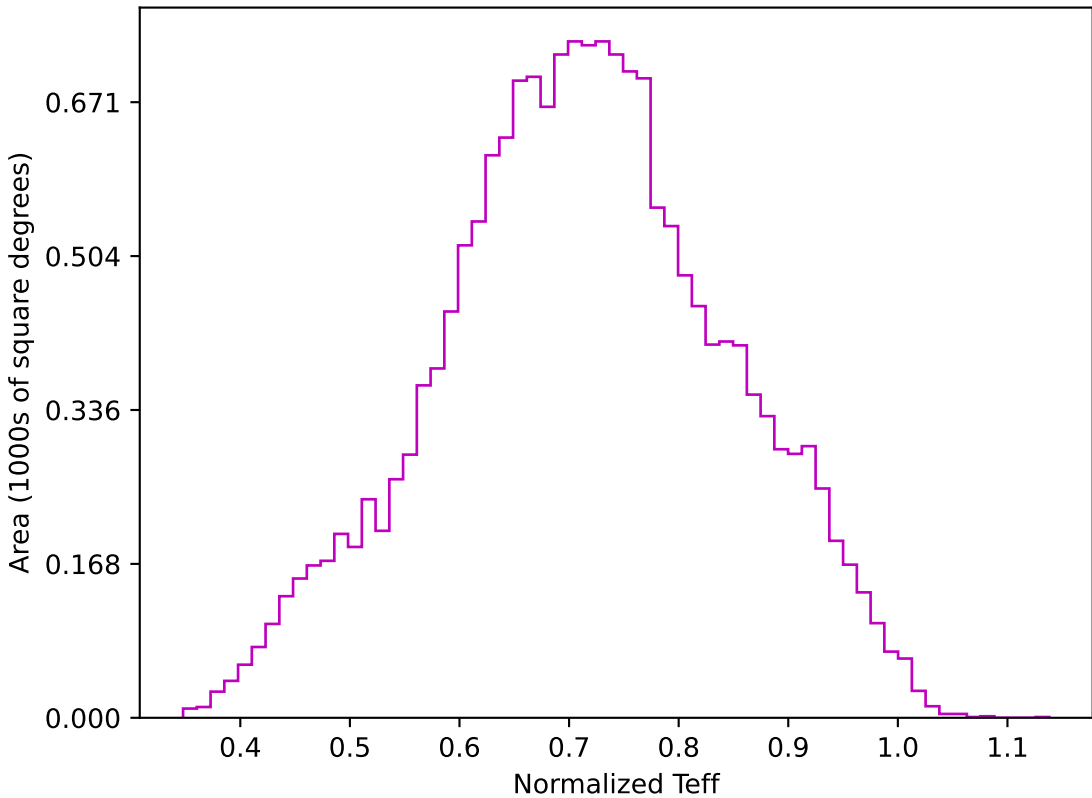
too_elab_r8_d2_gz_v3.4_10yrs WFD z band: Normalized Teff
