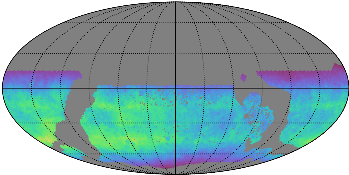
too_elab_r8_d2_gz_v3.4_10yrs WFD y band: Normalized Teff
