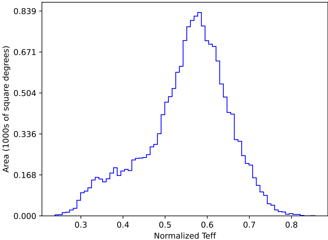
too_elab_r8_d2_gz_v3.4_10yrs WFD y band: Normalized Teff
