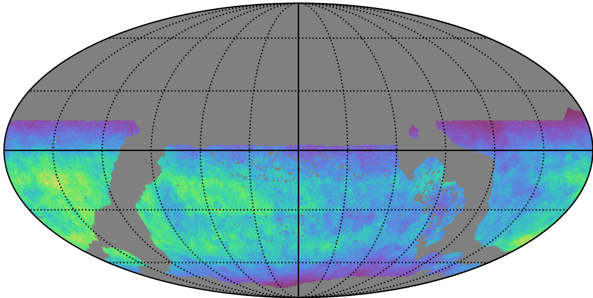
too_elab_r8_d2_gz_v3.4_10yrs WFD u band: Normalized Teff
