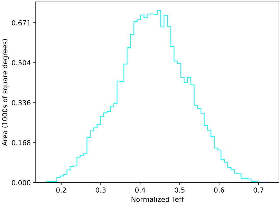
too_elab_r8_d2_gz_v3.4_10yrs WFD u band: Normalized Teff
