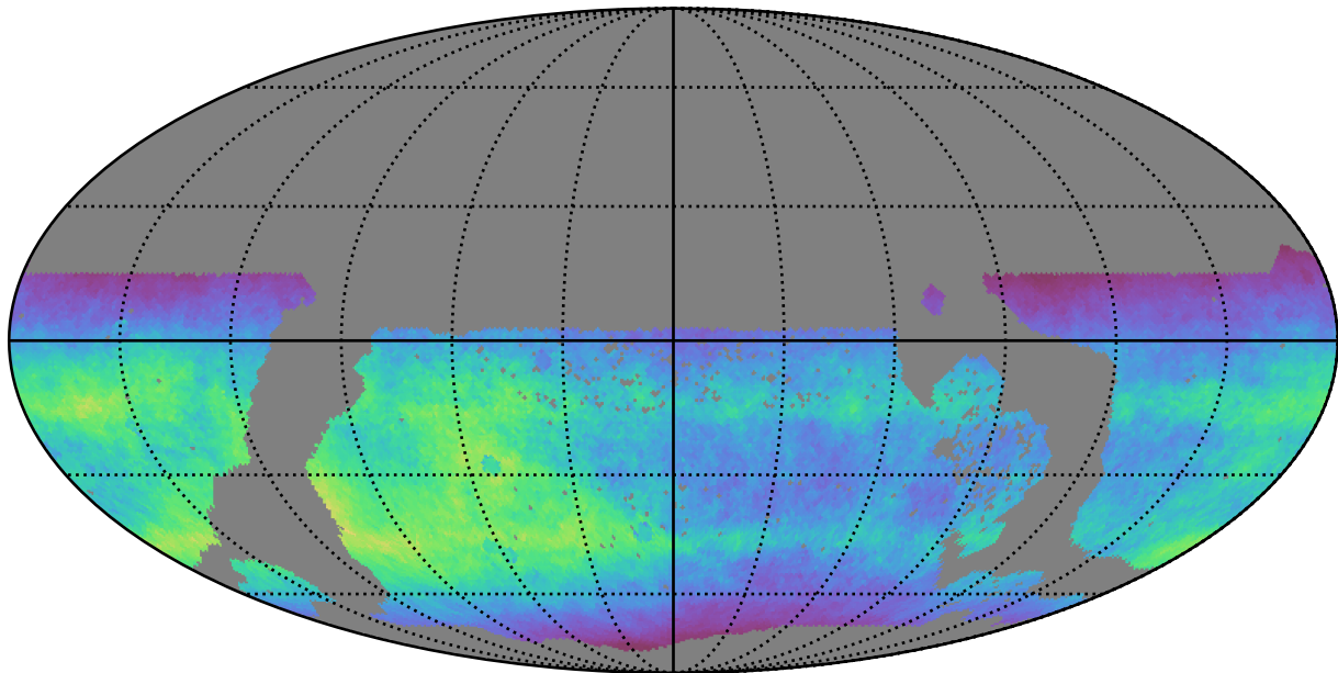
too_elab_r8_d2_gz_v3.4_10yrs WFD i band: Normalized Teff
