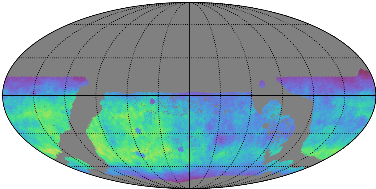
too_elab_r8_d2_gz_v3.4_10yrs WFD g band: Normalized Teff
