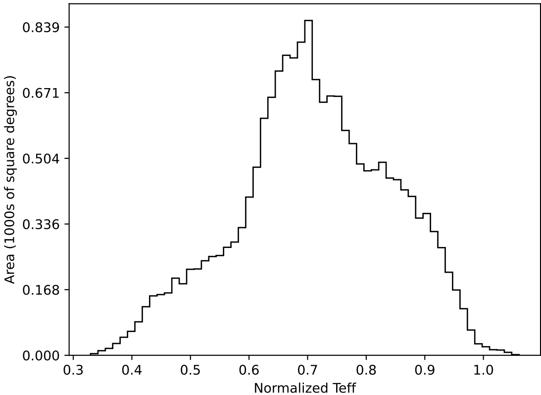
too_elab_r8_d2_gz_v3.4_10yrs WFD all bands: Normalized Teff
