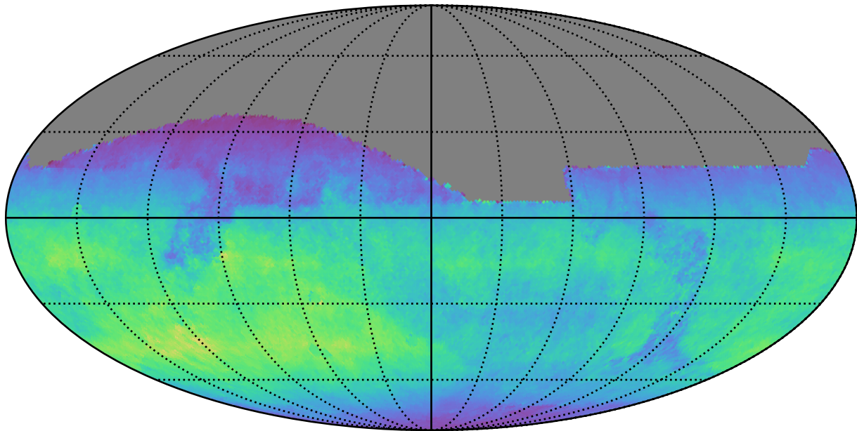
too_elab_r8_d2_gz_v3.4_10yrs All sky z band: Normalized Teff
