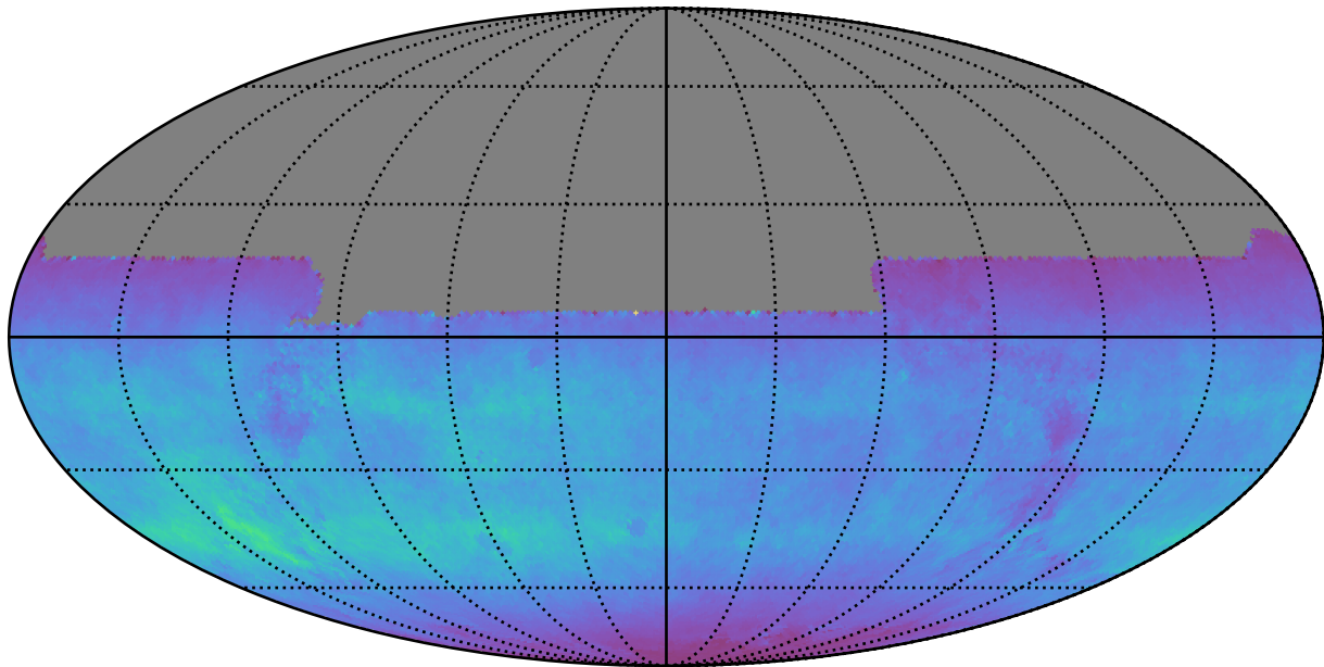
too_elab_r8_d2_gz_v3.4_10yrs All sky y band: Normalized Teff
