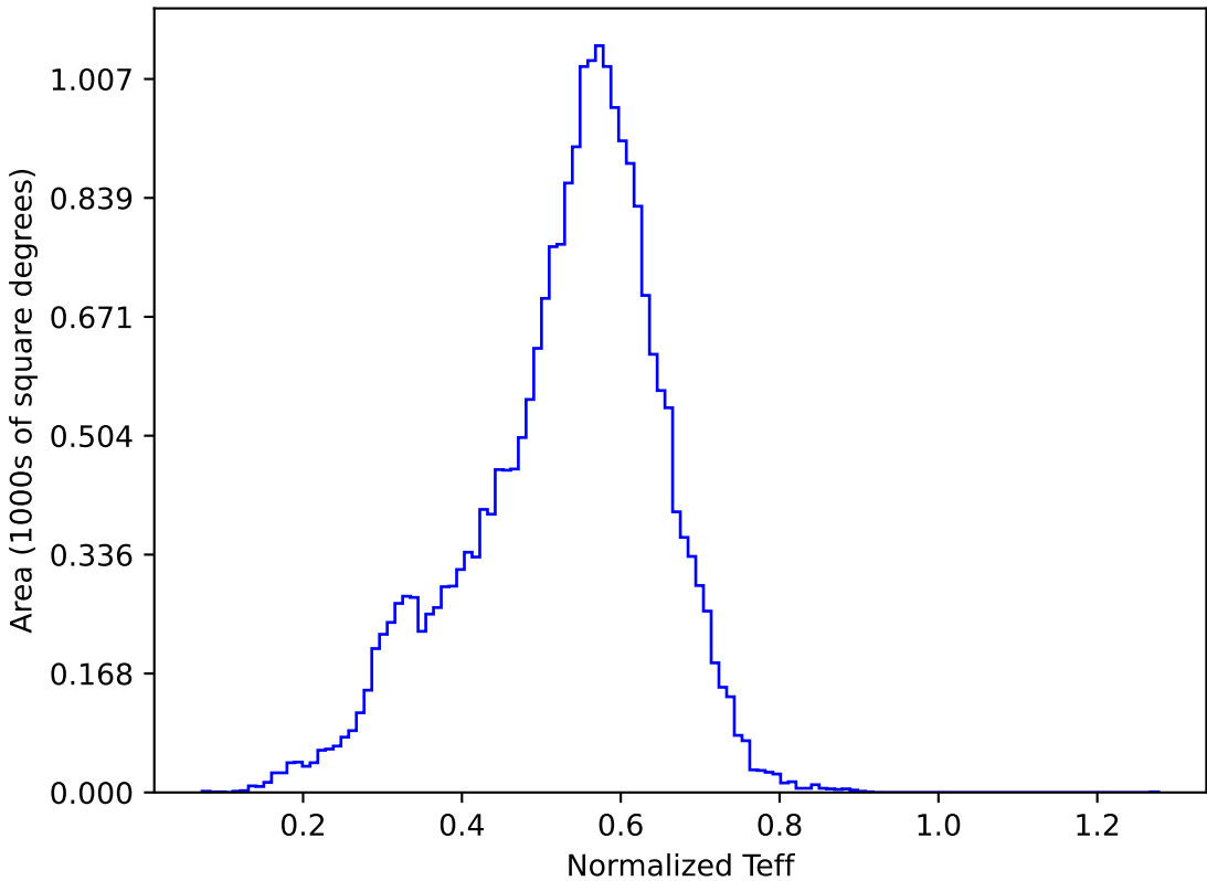
too_elab_r8_d2_gz_v3.4_10yrs All sky y band: Normalized Teff
