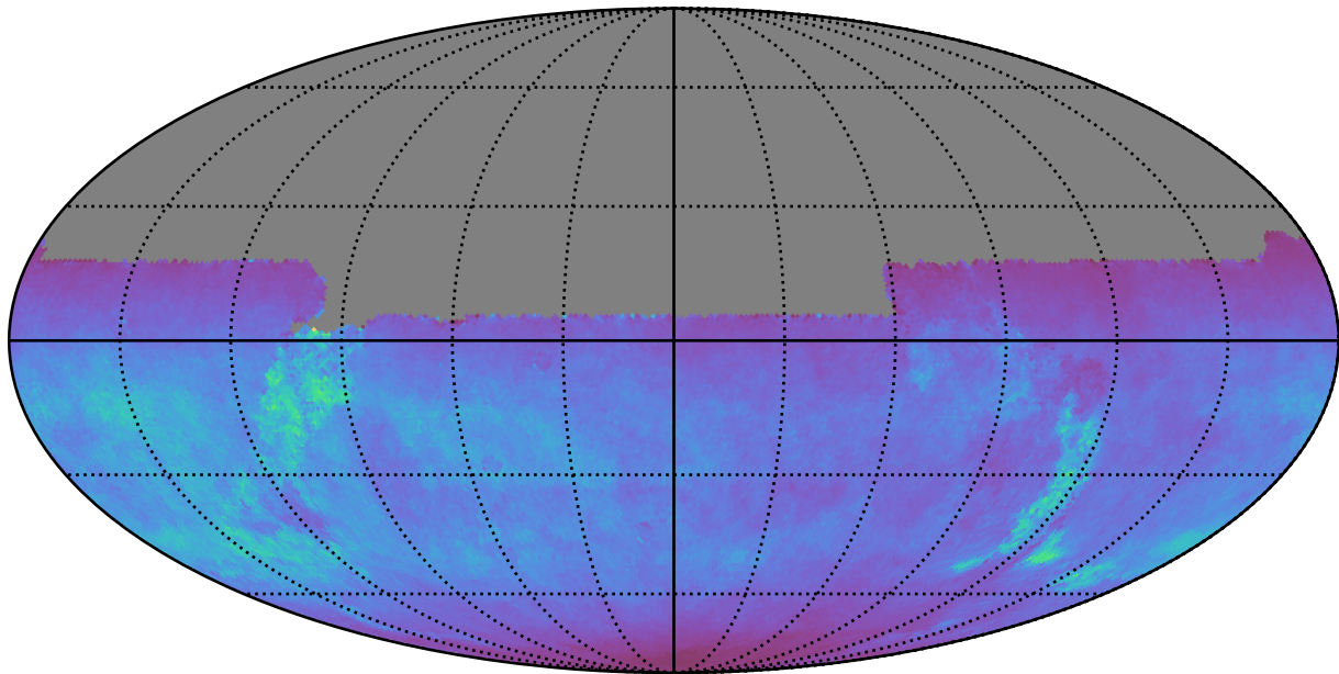
too_elab_r8_d2_gz_v3.4_10yrs All sky u band: Normalized Teff
