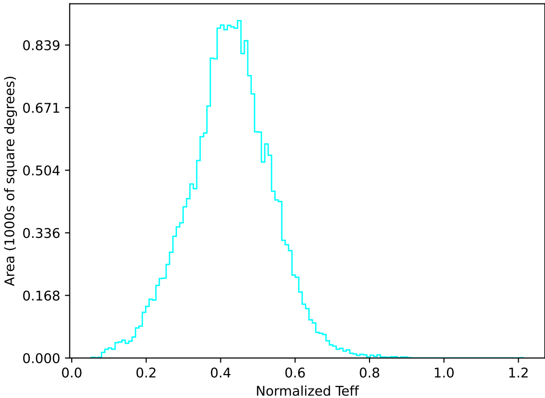
too_elab_r8_d2_gz_v3.4_10yrs All sky u band: Normalized Teff
