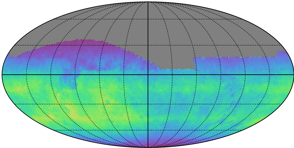
too_elab_r8_d2_gz_v3.4_10yrs All sky i band: Normalized Teff
