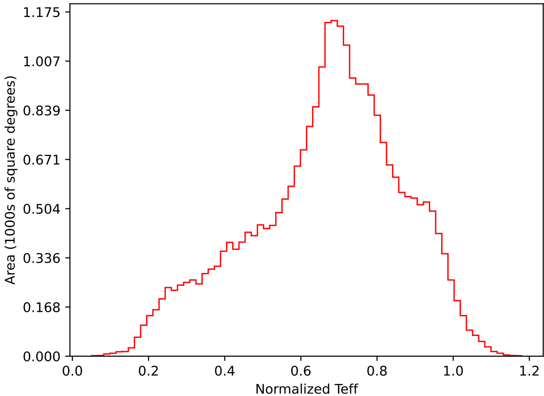
too_elab_r8_d2_gz_v3.4_10yrs All sky i band: Normalized Teff
