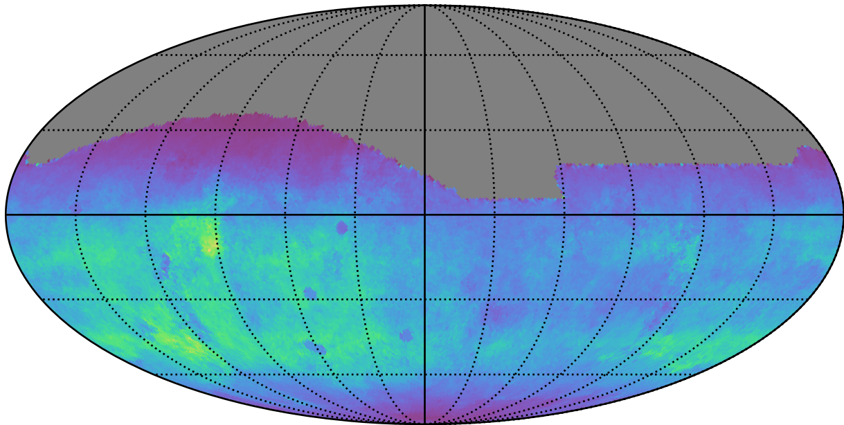
too_elab_r8_d2_gz_v3.4_10yrs All sky g band: Normalized Teff
