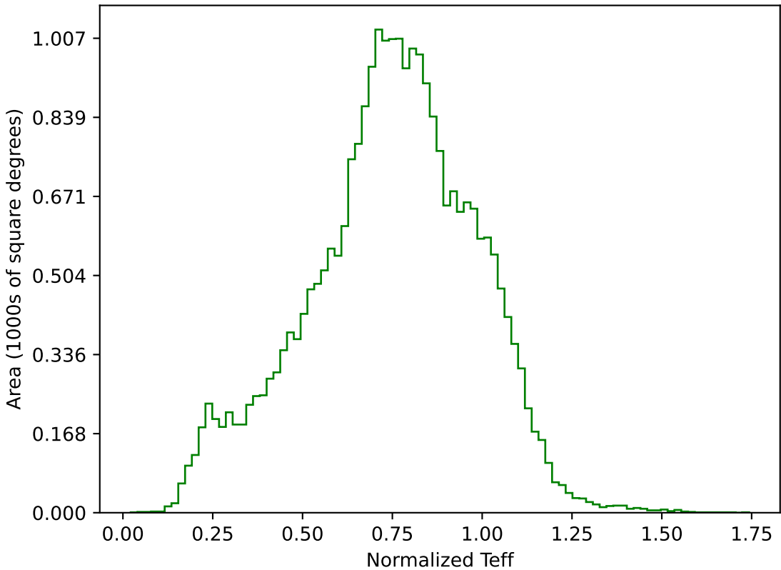
too_elab_r8_d2_gz_v3.4_10yrs All sky g band: Normalized Teff
