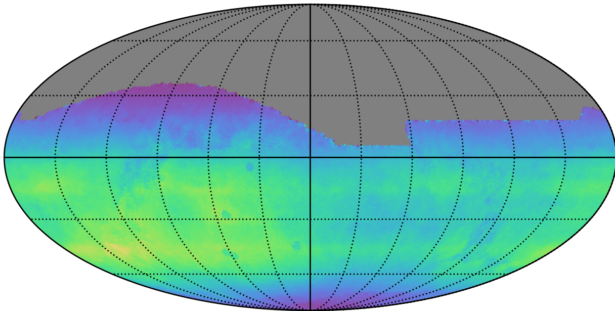
too_elab_r8_d2_gz_v3.4_10yrs All sky all bands: Normalized Teff
