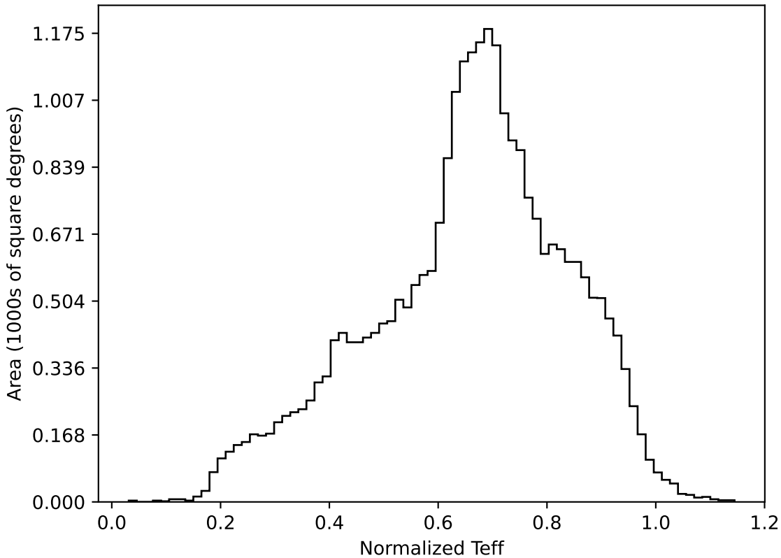
too_elab_r8_d2_gz_v3.4_10yrs All sky all bands: Normalized Teff
