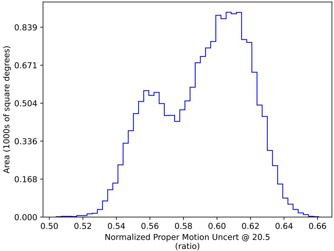
too_elab_r8_d2_gz_v3.4_10yrs WFD: Normalized Proper Motion Uncert @ 20.5
