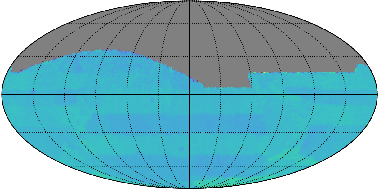
too_elab_r8_d2_gz_v3.4_10yrs All sky: Normalized Proper Motion Uncert @ 20.5
