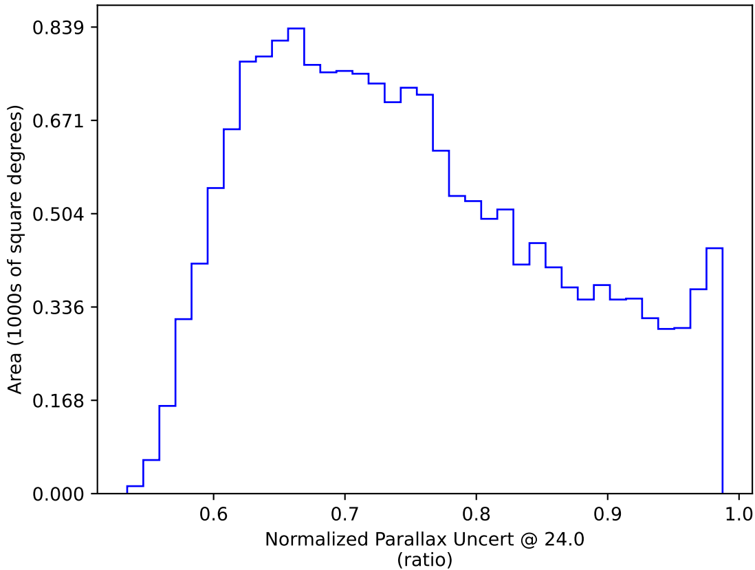
too_elab_r8_d2_gz_v3.4_10yrs WFD: Normalized Parallax Uncert @ 24.0
