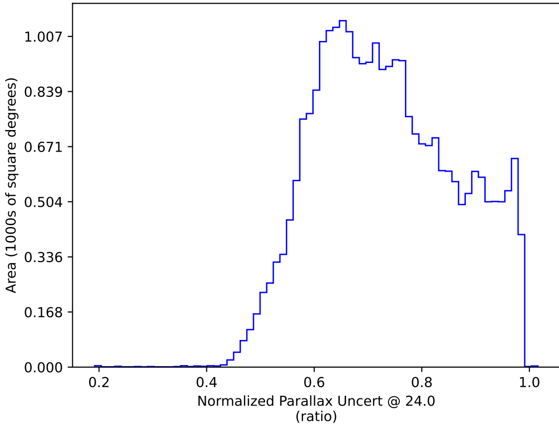
too_elab_r8_d2_gz_v3.4_10yrs All sky: Normalized Parallax Uncert @ 24.0
