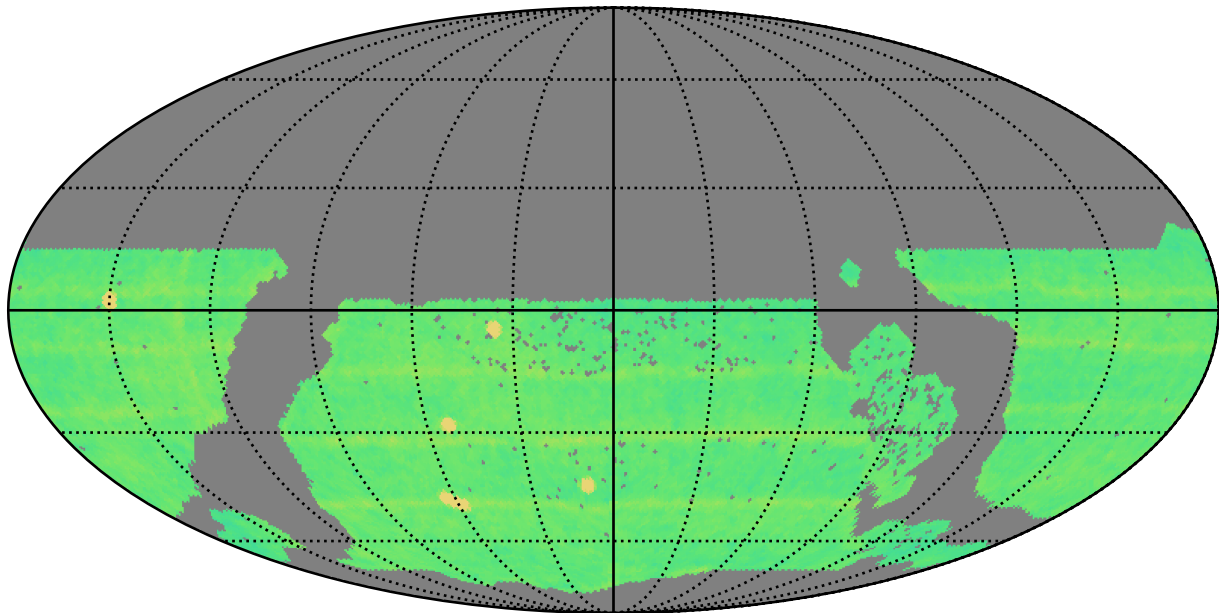
too_elab_r8_d2_gz_v3.4_10yrs WFD all bands: N Unique Nights
