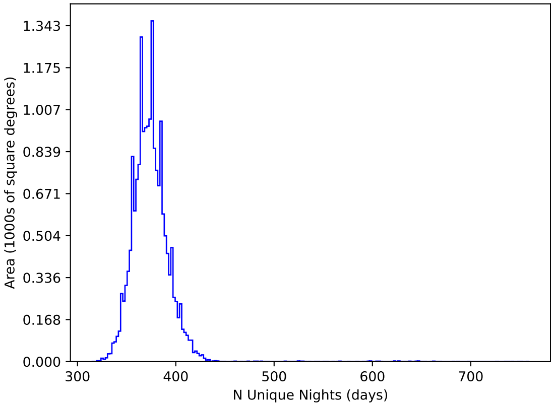
too_elab_r8_d2_gz_v3.4_10yrs WFD all bands: N Unique Nights
