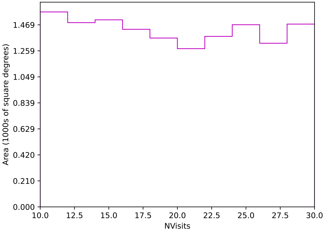
too_elab_r8_d2_gz_v3.4_10yrs Yr 3-4 z band: NVisits
