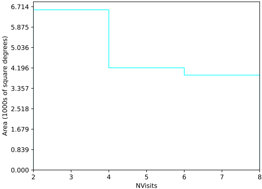
too_elab_r8_d2_gz_v3.4_10yrs Yr 3-4 u band: NVisits
