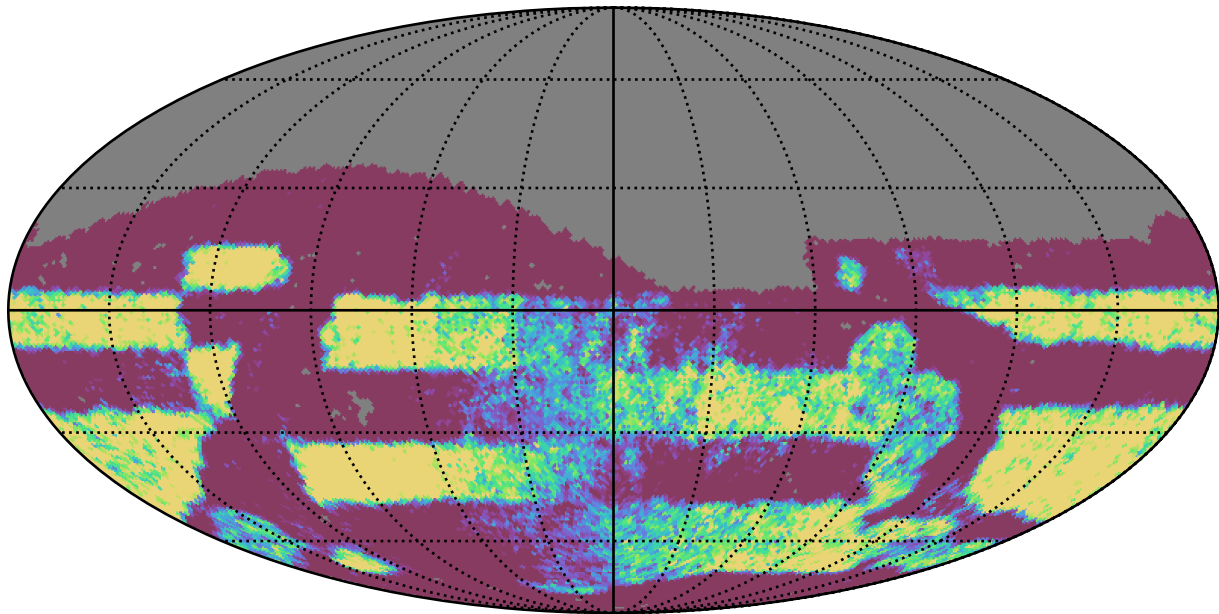
too_elab_r8_d2_gz_v3.4_10yrs Yr 3-4 r band: NVisits
