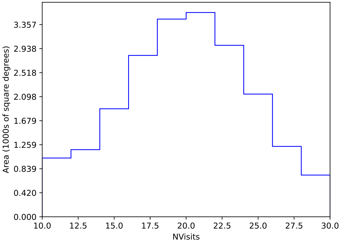
too_elab_r8_d2_gz_v3.4_10yrs Yr 1 y band: NVisits
