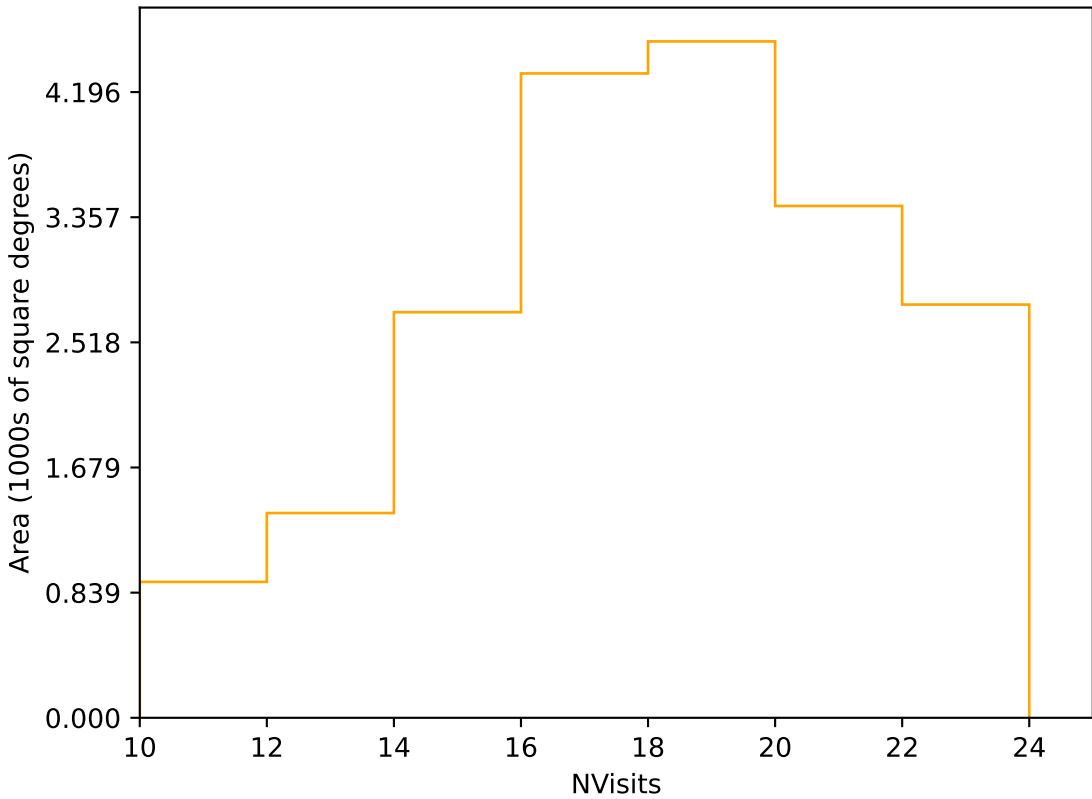
too_elab_r8_d2_gz_v3.4_10yrs Yr 1 r band: NVisits
