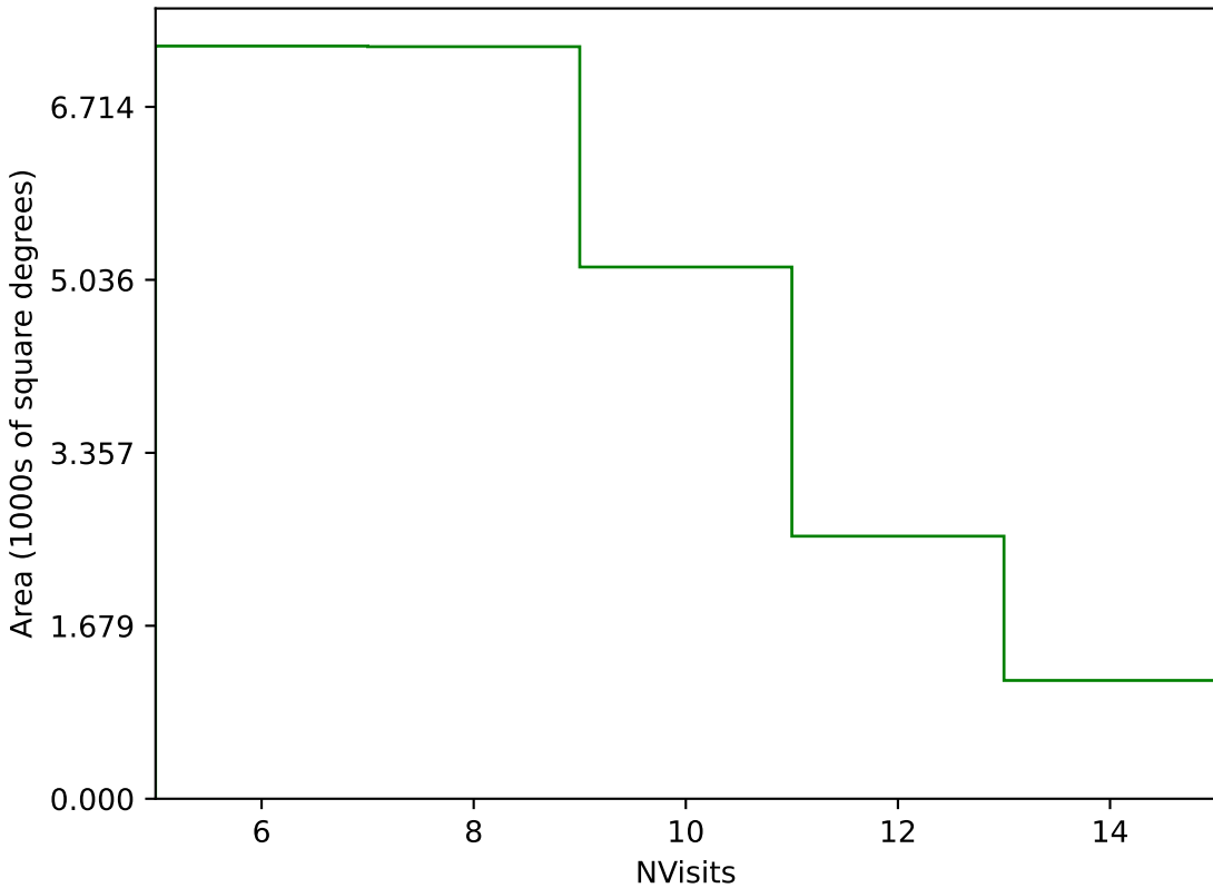
too_elab_r8_d2_gz_v3.4_10yrs Yr 1 g band: NVisits
