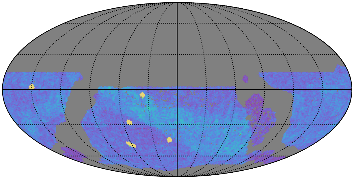
too_elab_r8_d2_gz_v3.4_10yrs WFD z band: NVisits
