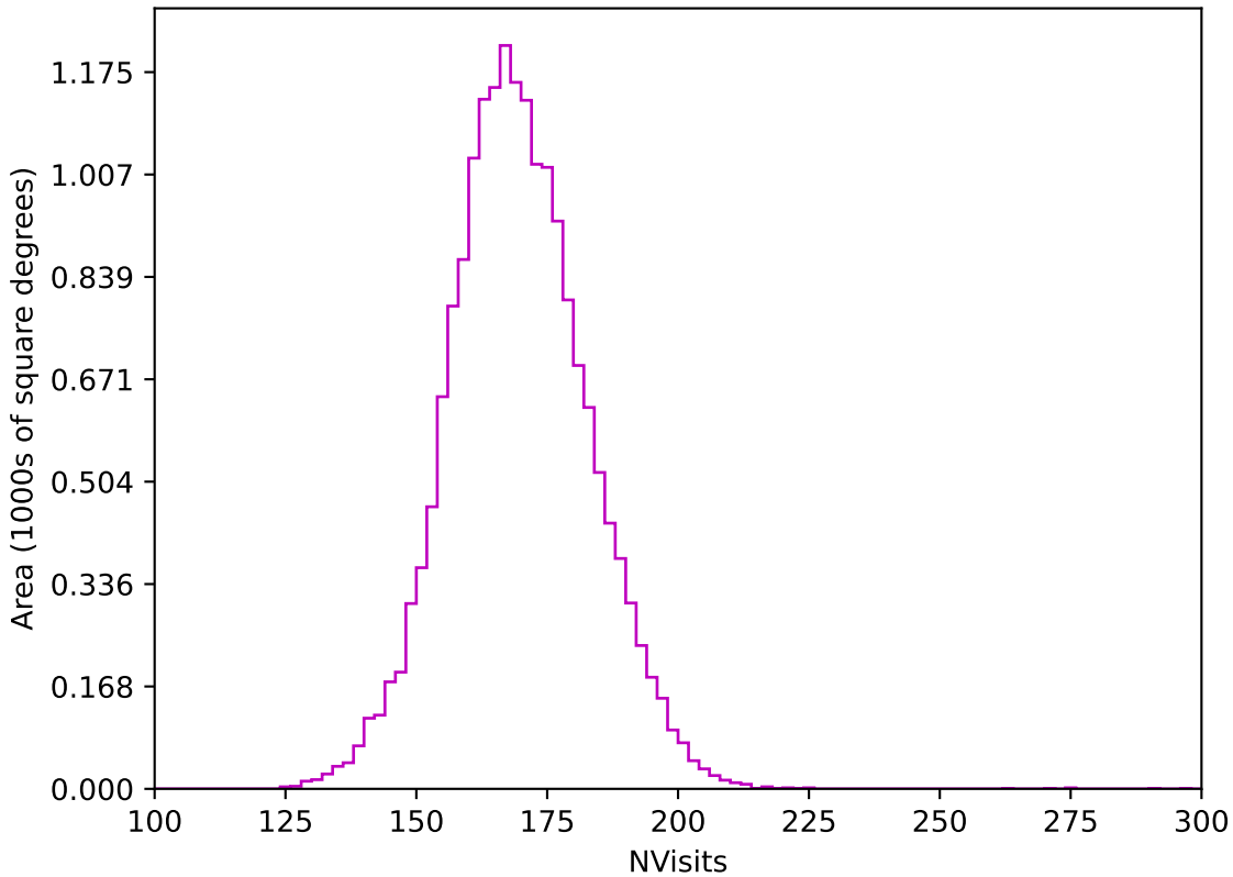
too_elab_r8_d2_gz_v3.4_10yrs WFD z band: NVisits
