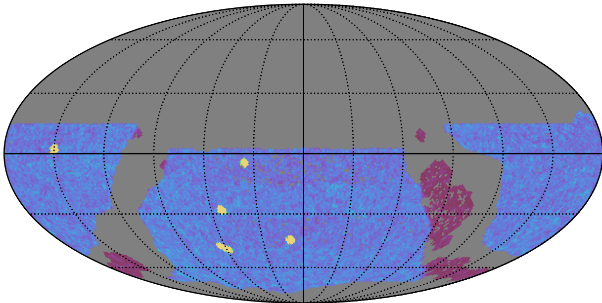
too_elab_r8_d2_gz_v3.4_10yrs WFD y band: NVisits
