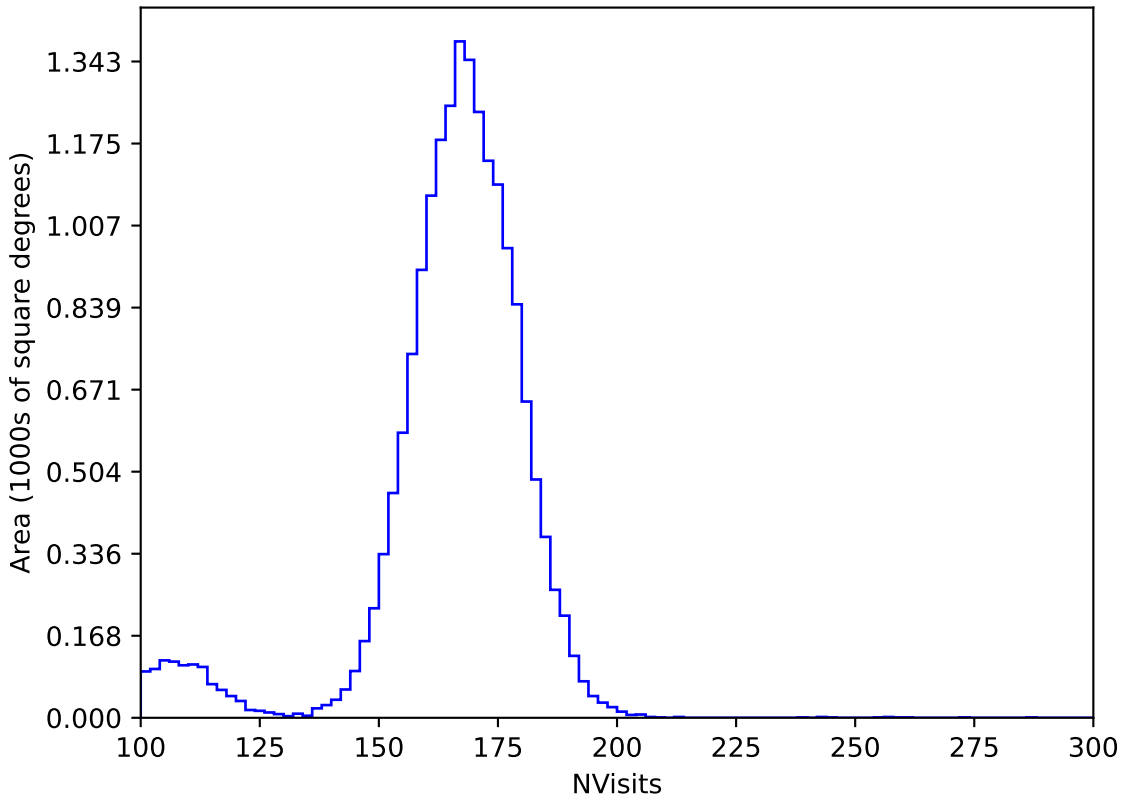
too_elab_r8_d2_gz_v3.4_10yrs WFD y band: NVisits
