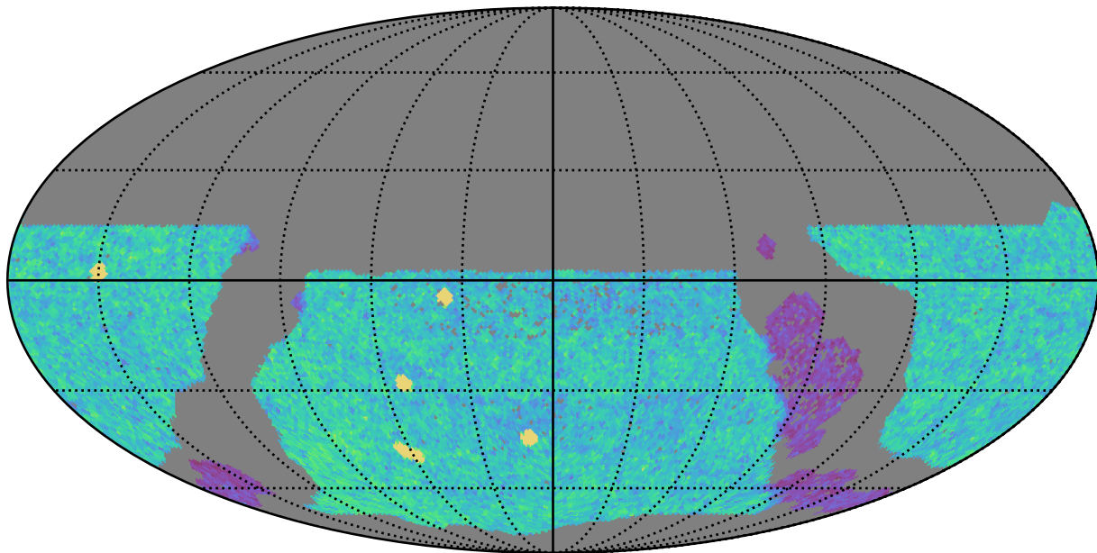
too_elab_r8_d2_gz_v3.4_10yrs WFD u band: NVisits
